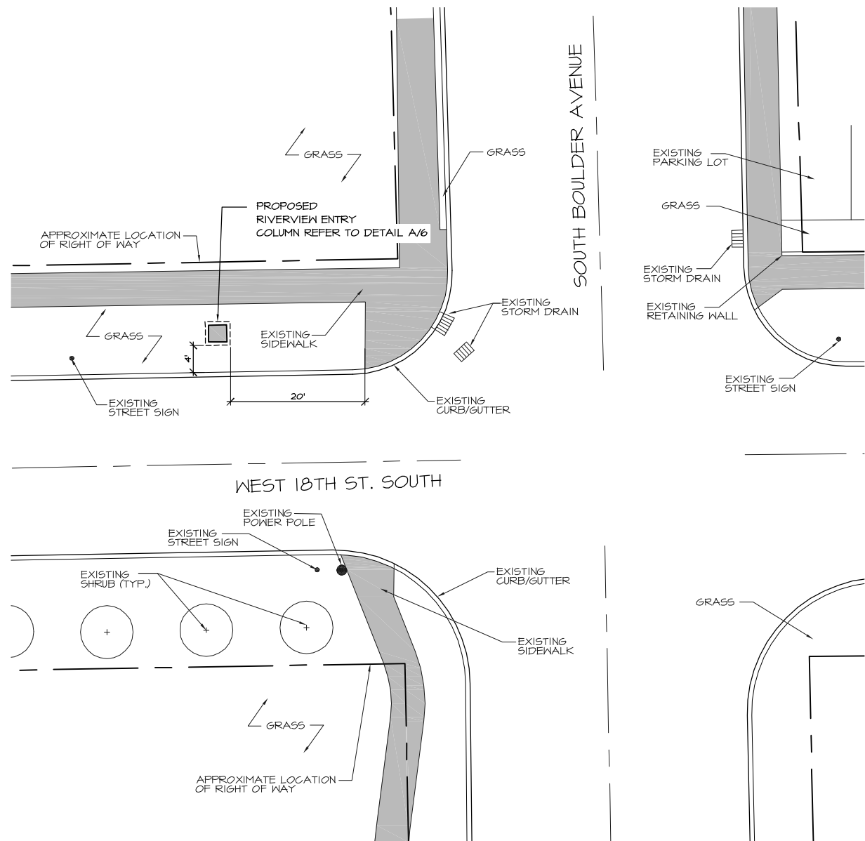
3 PLAN: INTERSECTION OF W. 18TH ST. S. & S. BOULDER AVE. SCALE: 1" = 10'-0"
